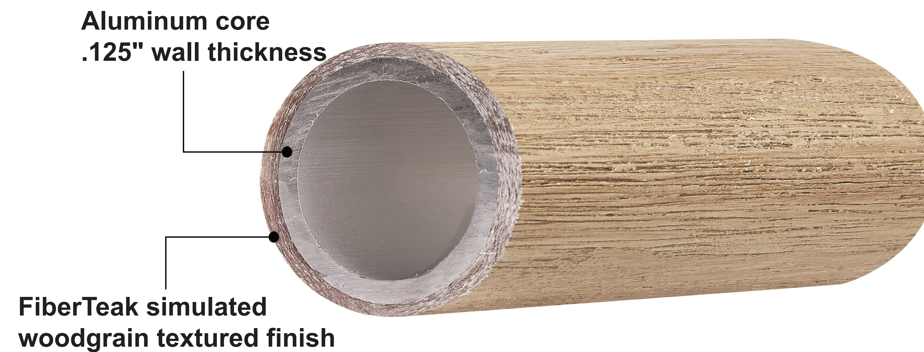
DETAIL A INTERNAL VIEW OF POLE CONSTRUCTION
