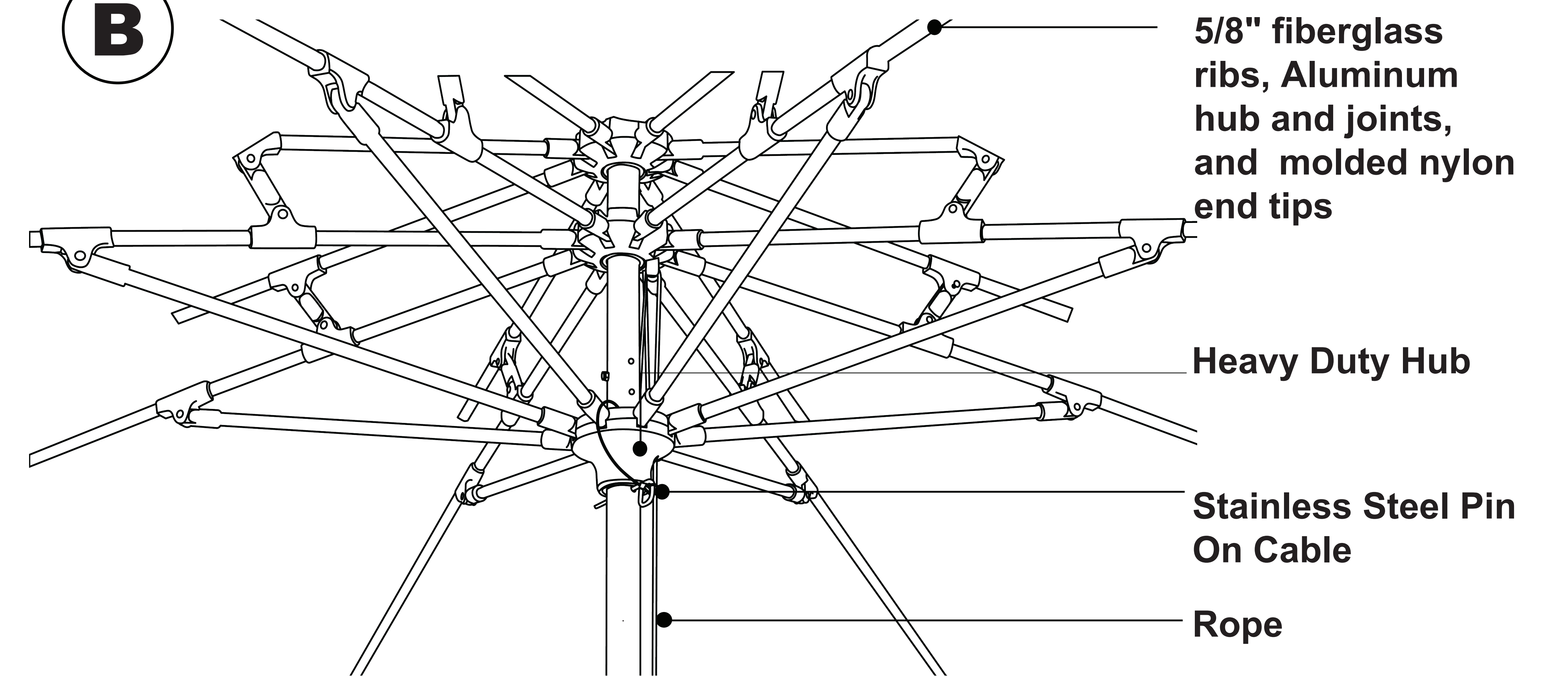
DETAIL B RIB, HUB AND PULLEY ASSEMBLY
